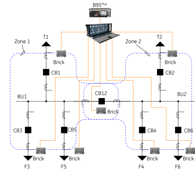
Two single buses with a bus coupler
