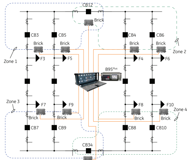
Breaker-and-a-half arrangement
