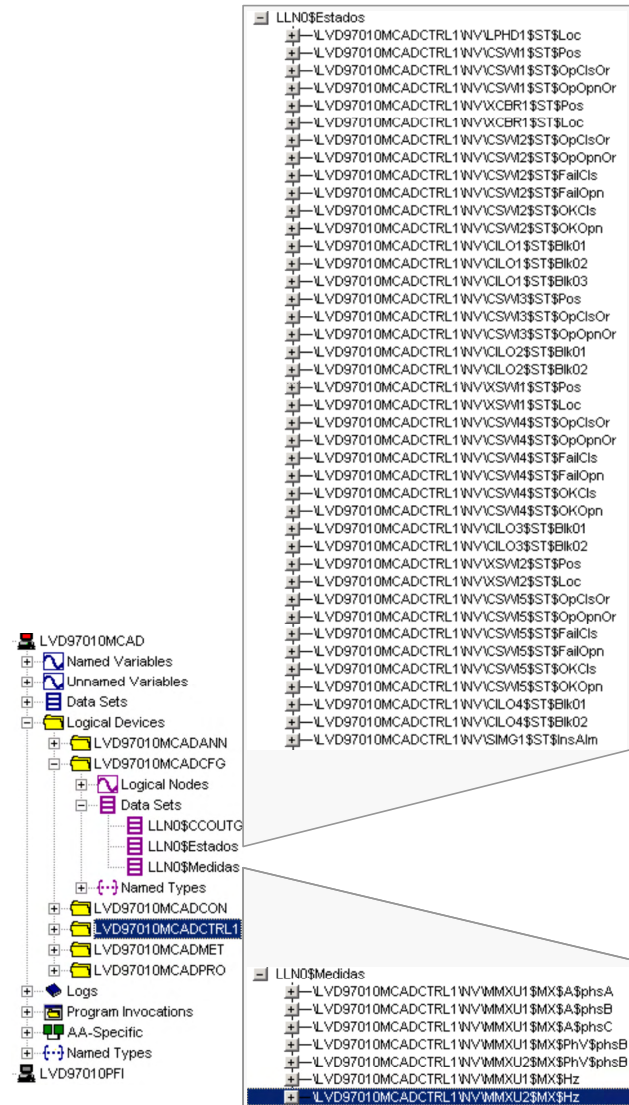
Fig. 10. Required IED data sets and their contents
