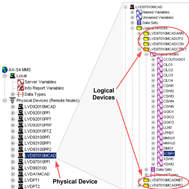
Fig. 9. Browsing on physical devices, logical devices, and logical nodes
